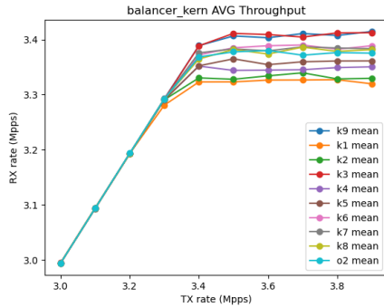
(j) xdp-balancer: Throughput vs. Offered load
