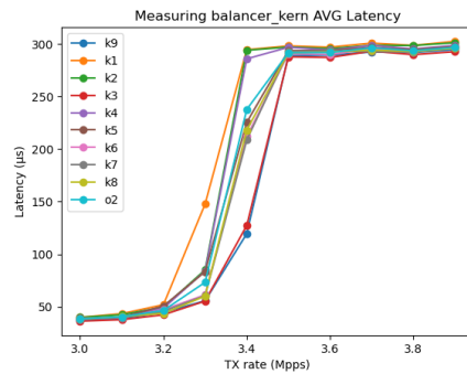
(k) xdp-balancer: Avg. latency vs. Offered load
